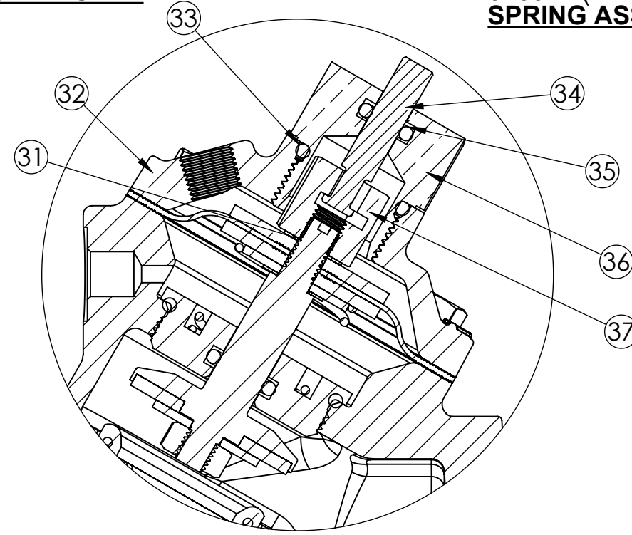
1070144 (V42B-0021-00000) (3/4' NPT) 1072648 (V42C-0021-00000) (1" NPT) POSITION INDICATOR MODEL
