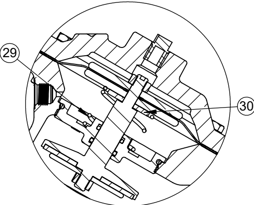
1072932 (V42G-0001-00000) (2"NPT) 1072994 (V42H-0001-00000) (2 1/2" NPT) SPRING ASSIST OPEN
