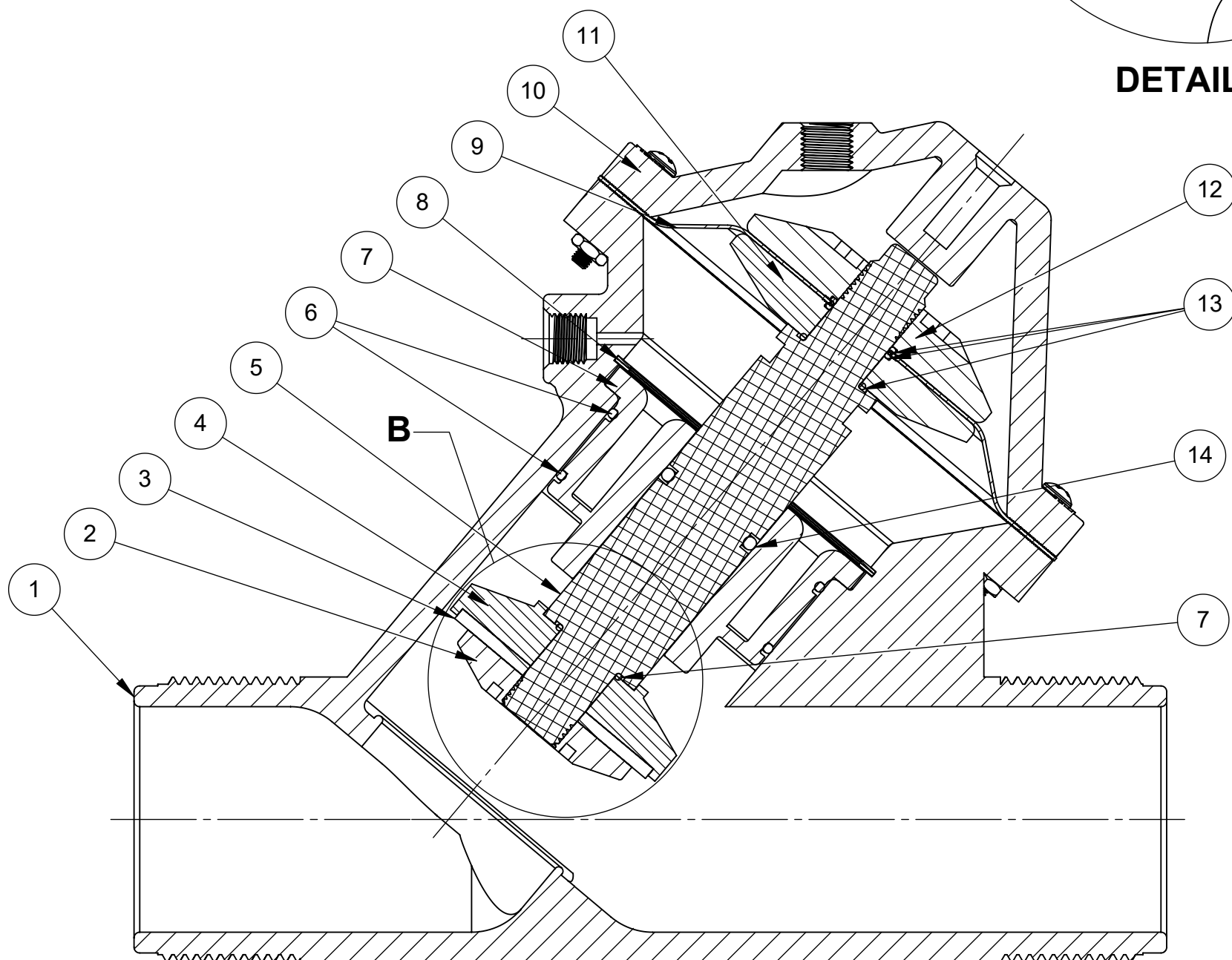
DETAIL C
