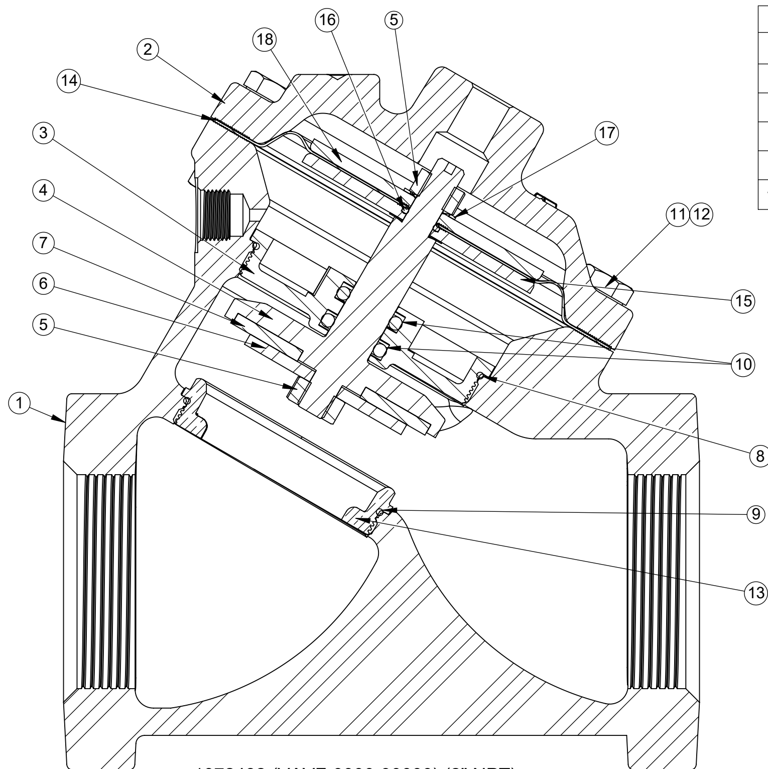
1072482 (VAVF-0000-90000) (2" NPT) NORMALLY OPEN (STANDARD)
