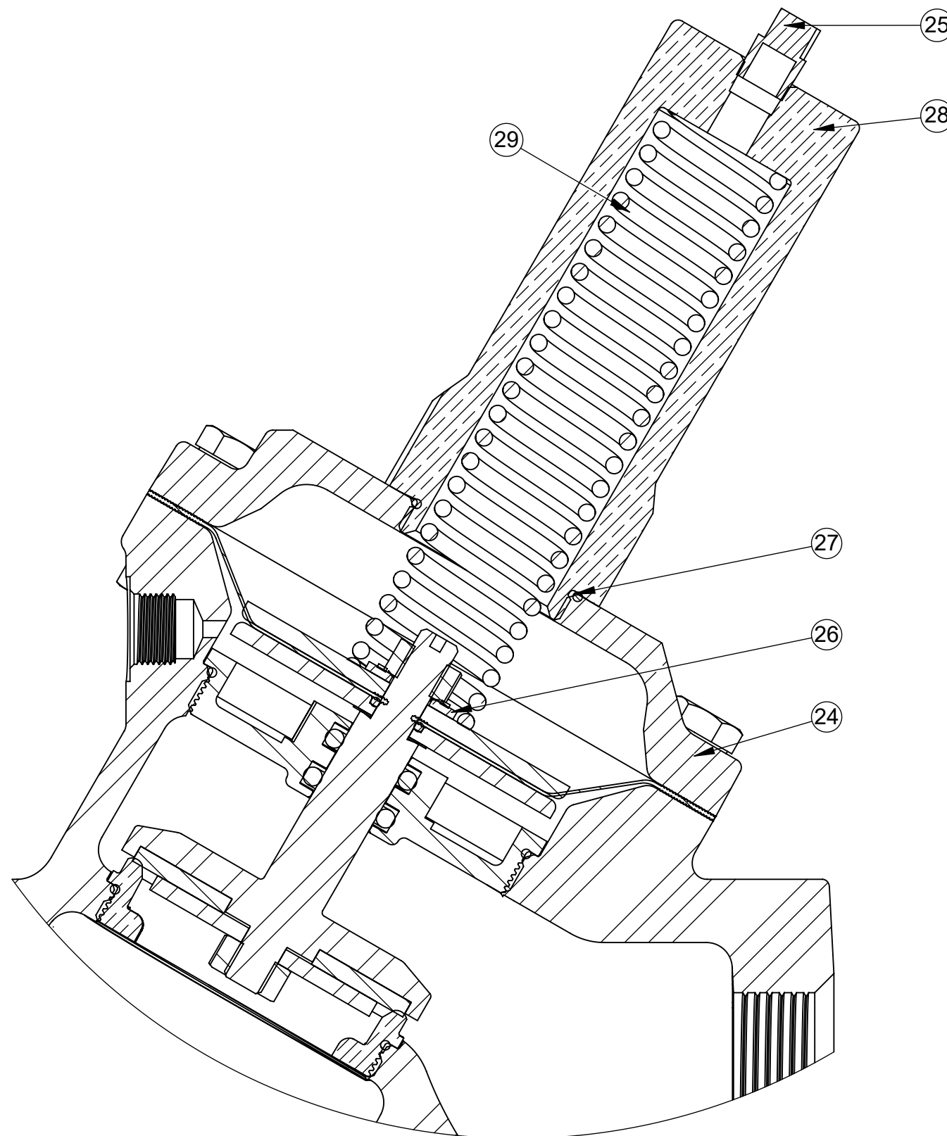
1072485 (VAVF-0002-90000) (2" NPT) SPRING ASSIST CLOSED
